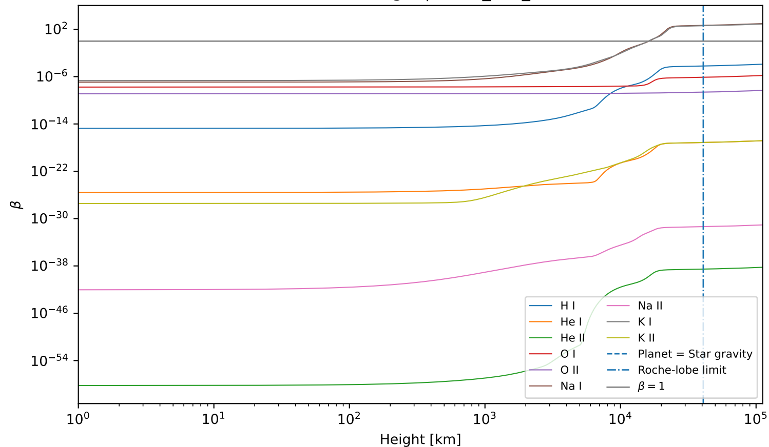
Beta vs height | WASP_121_b
